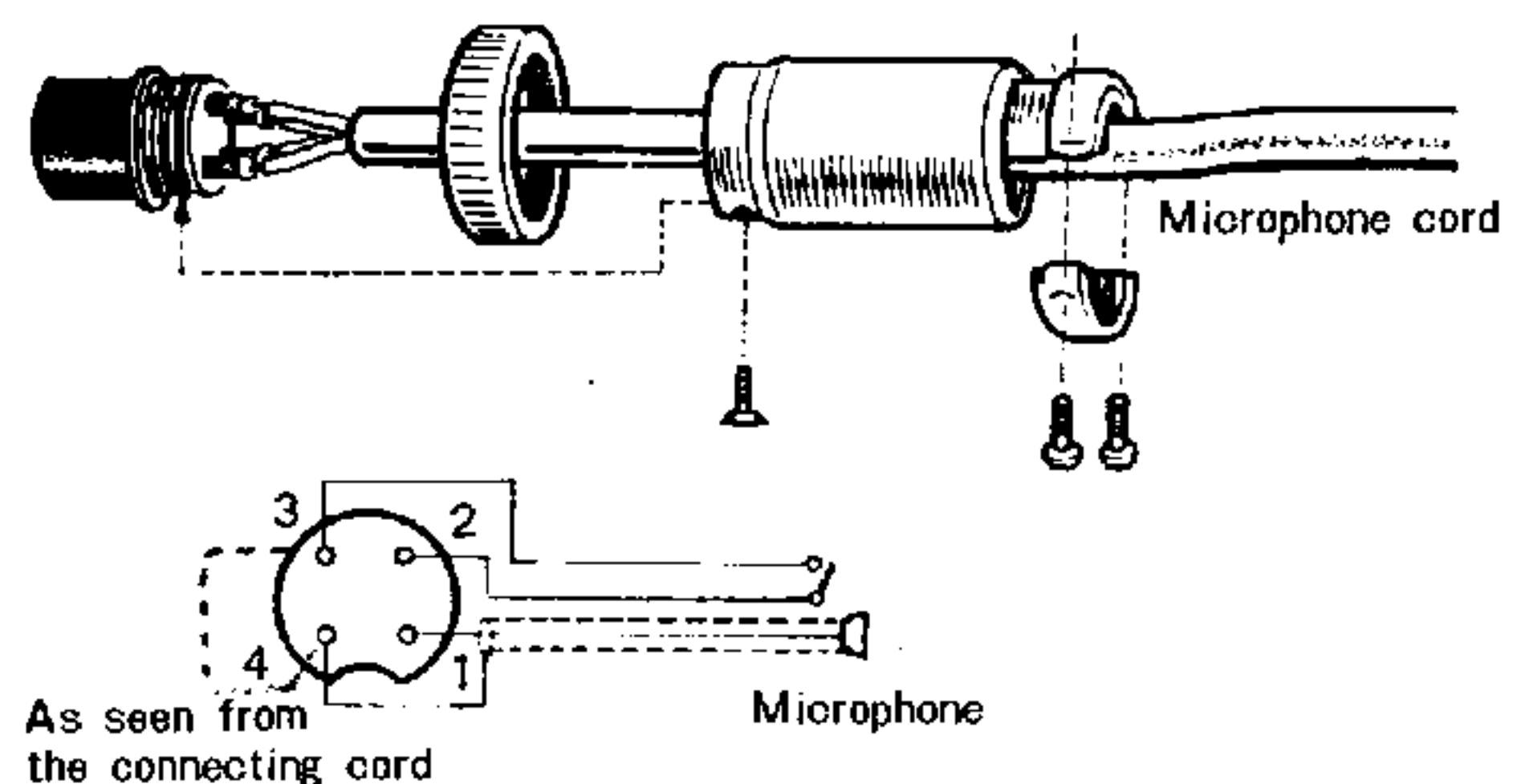
Fig. 13 Microphone cord connections
