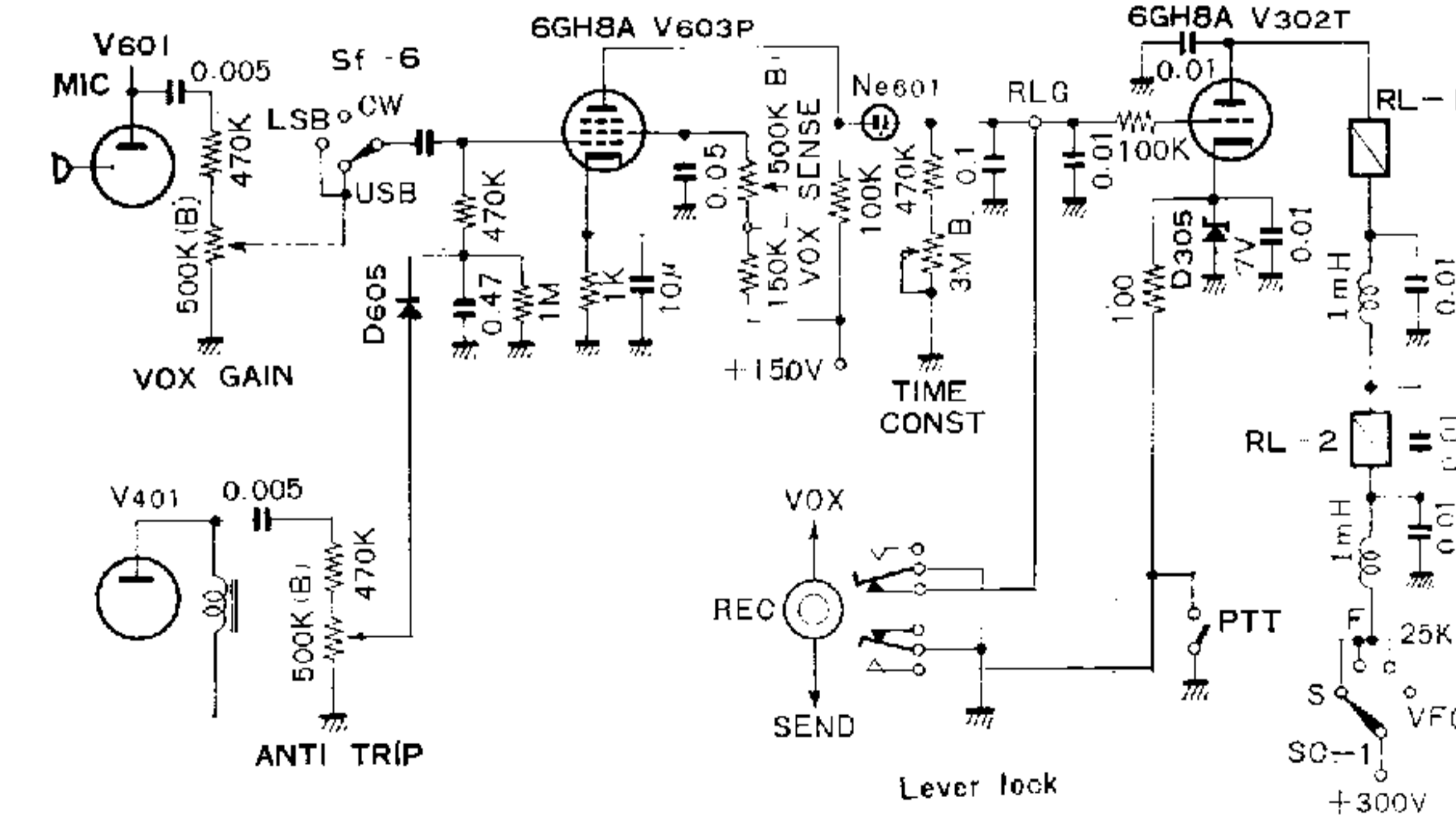
Fig. 8 VOX, anti-trip and relay amplifier
