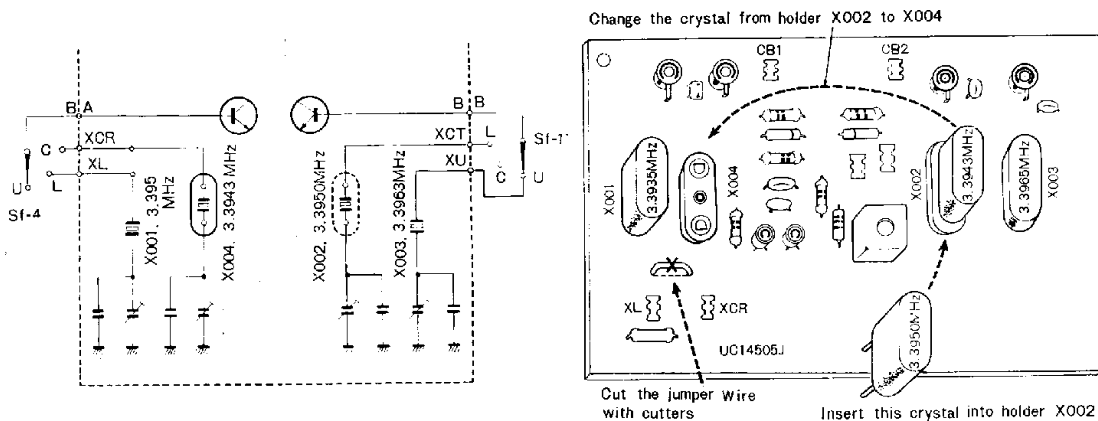
Fig. 18 Installing the crystal
