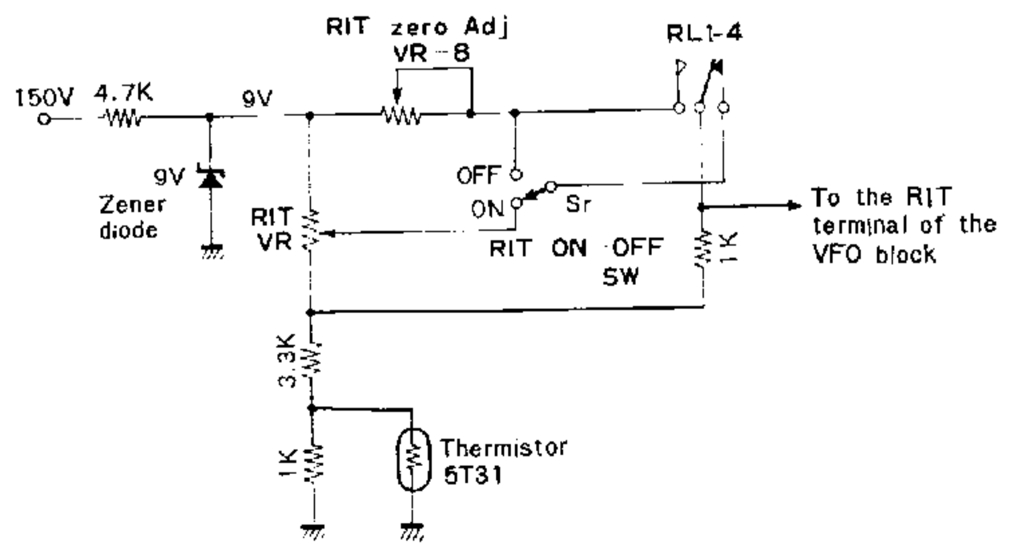
Fig. 6 RIT circuit
