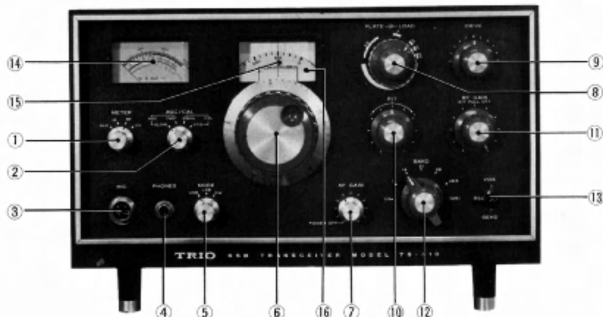
Photo 1 TS-510 Front Panel
