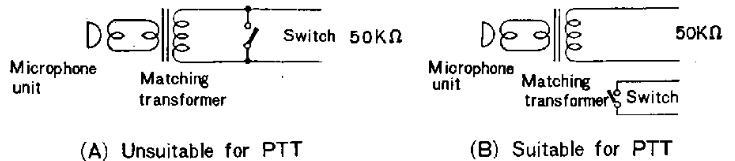
Fig. 12 Microphone with a switch
