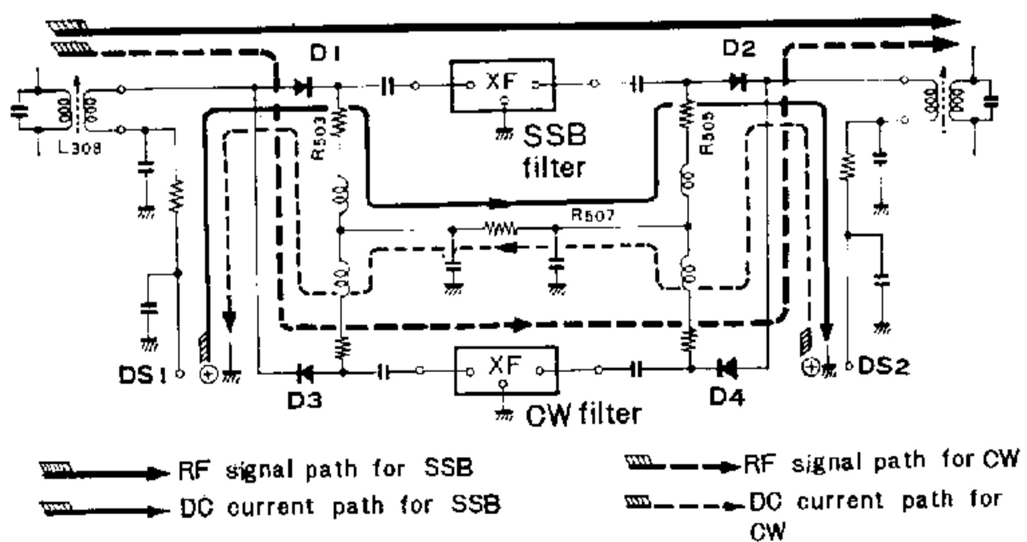
Fig. 5 Operation of diode switch
