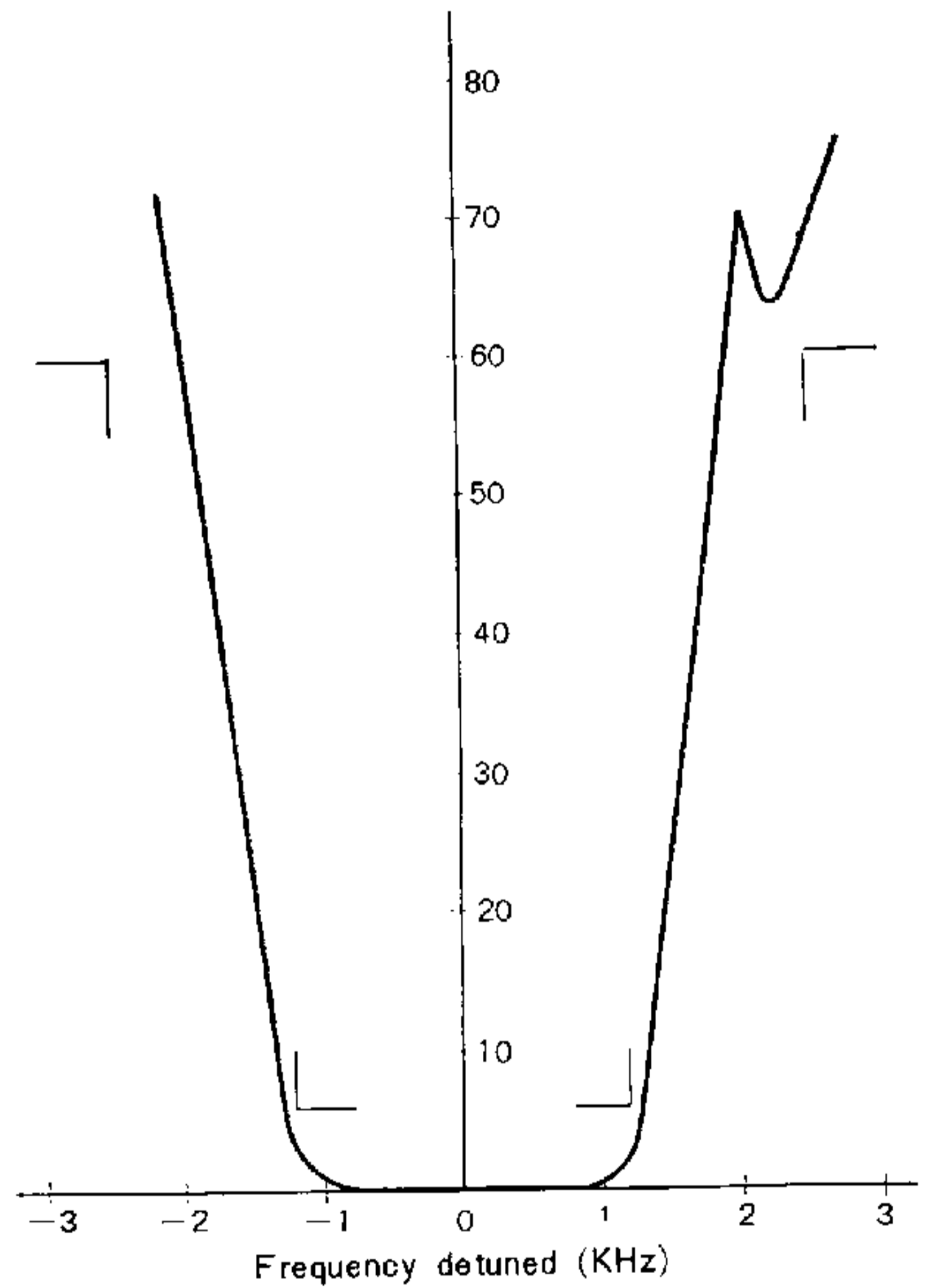
Fig. 4 SSB crystal filter characteristic curve
