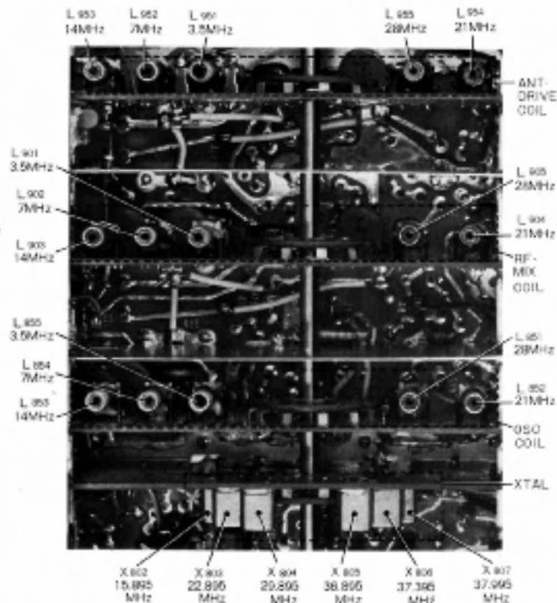
Fig. 23 Coil Pack
