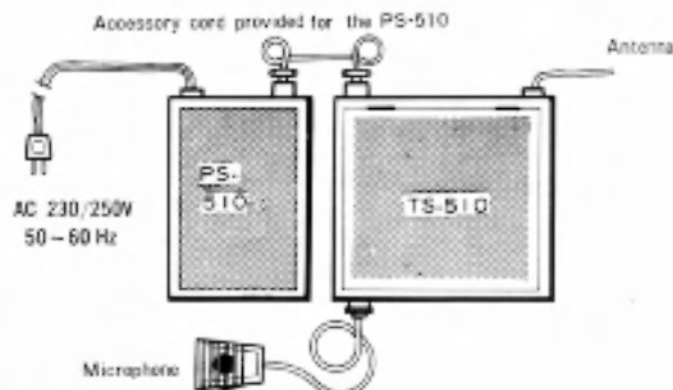
Fig. 10 TS-510 connections
