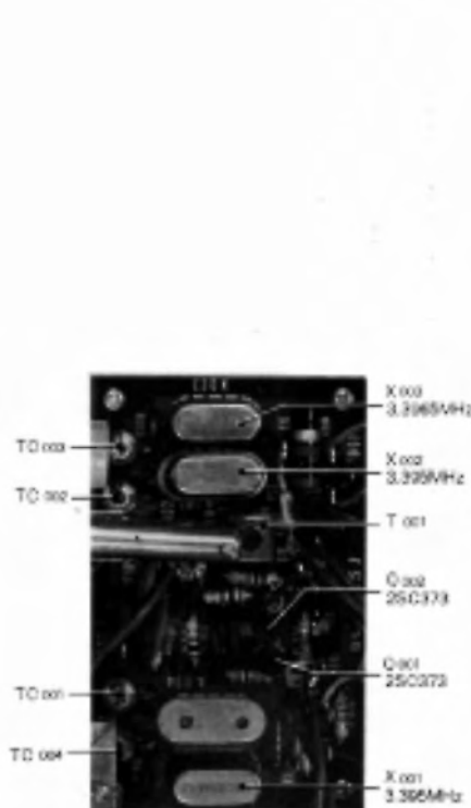
Fig. 21 Carrier Unit
