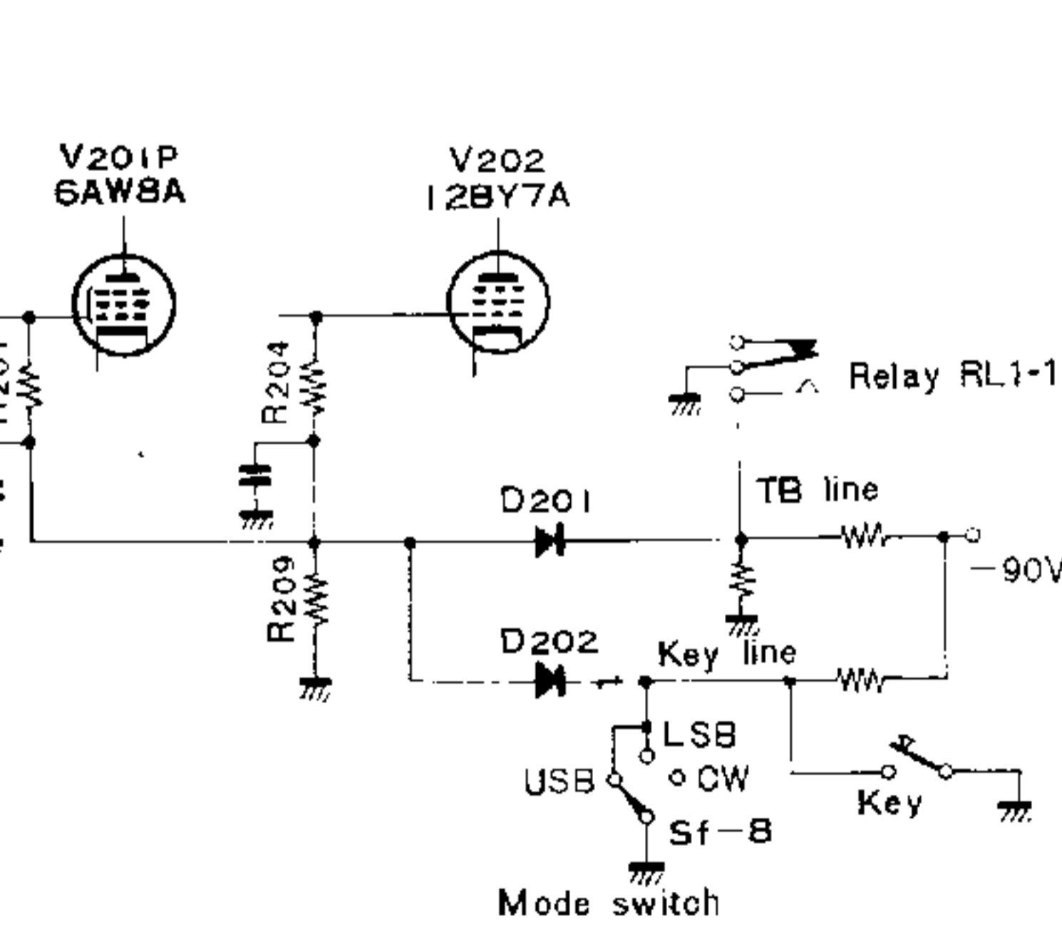
Fig. 7 Block bias keying circuit
