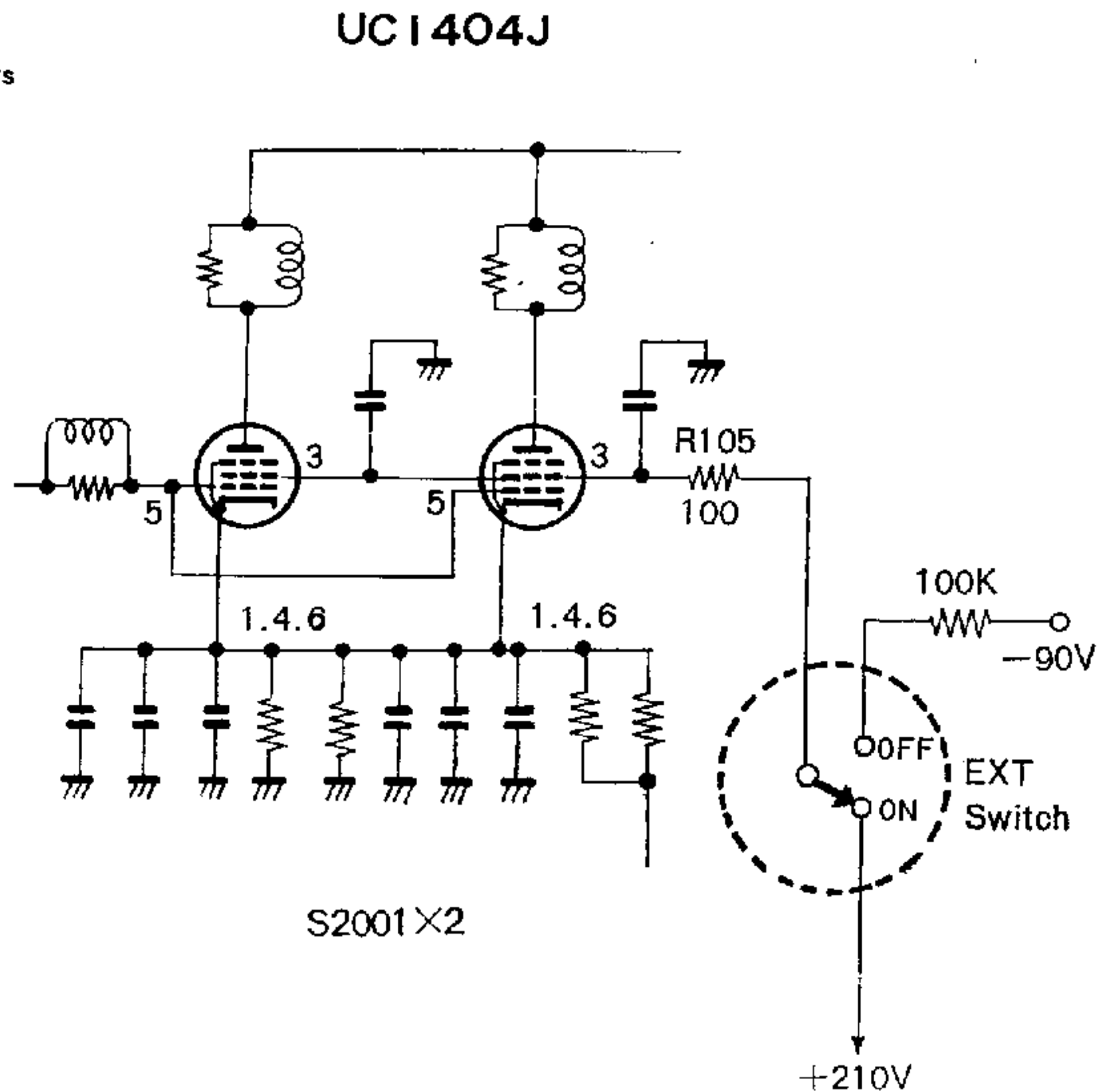
Fig. 20 Example use of the EXT switch
