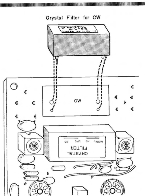
Fig. 17 Installing the CW Crystall Filter
