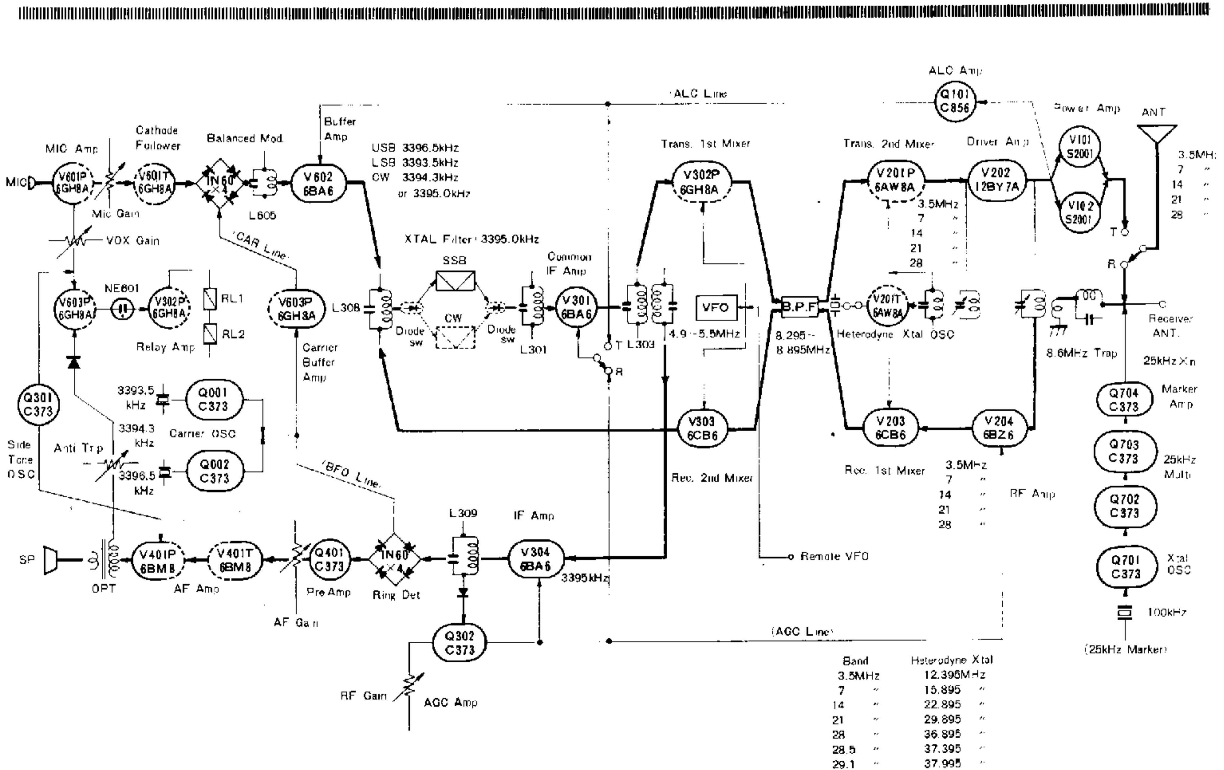
Fig. 1 Block Diagram
