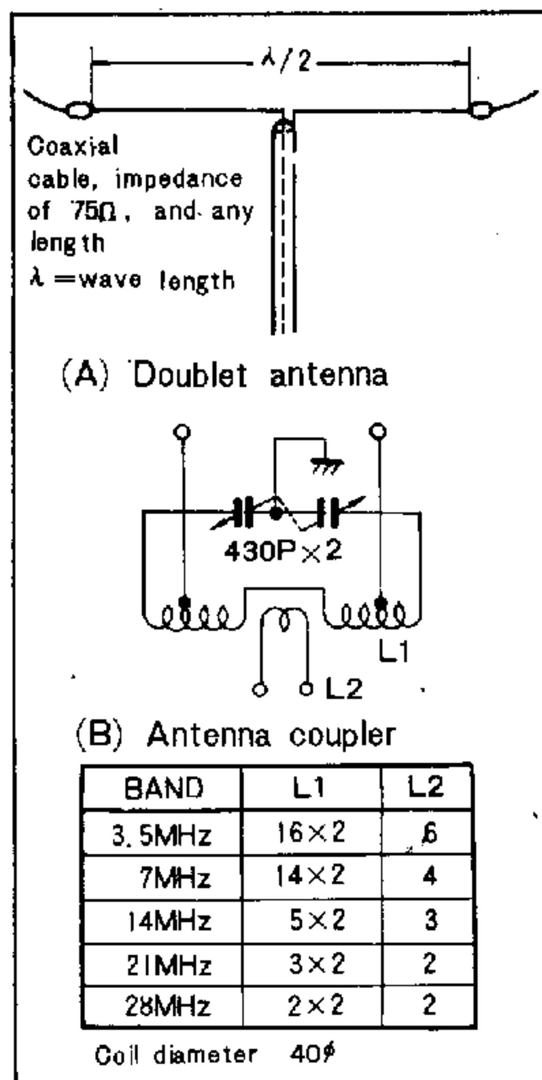
Fig. 11 Antenna coupler
